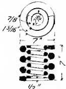
Figs. 4764-4765. Spring-caps (4).
